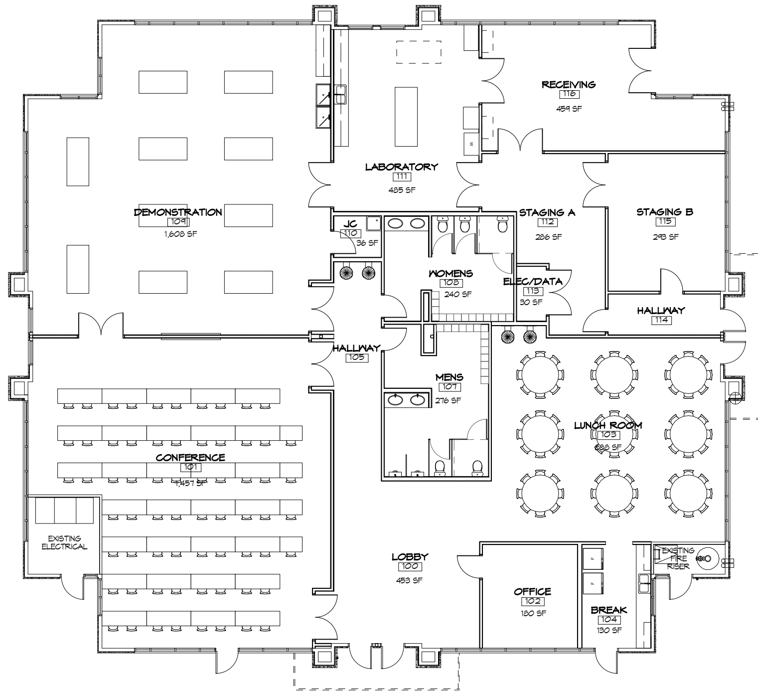
FLOOR PLAN
